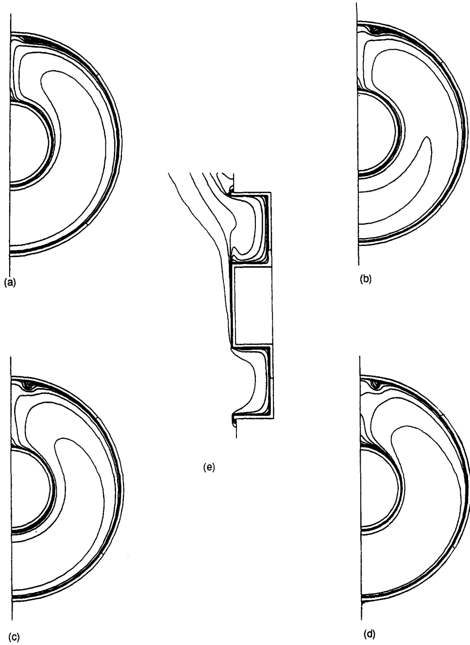
Fig. 9. Isotherms in different planes of the cavity; Ra^* = 3.71 \times 10^9 (range: 10^{-3} – 1.9 \times 10^{-2} , \Delta T = 2 \times 10^{-3} ), (a) z = L/4 , (b) z = L/2 , (c) z = 3L/4 , (d) z = L (aperture plane), (e) symmetry plane.
